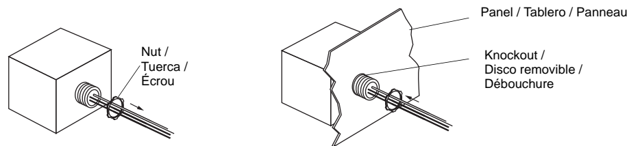
Figure / Figura / Figure 2 : Wiring / Alambrado / Câblage
